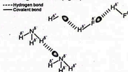
Figure: Hydrogen bonding in \text{NH}_3 and HF
