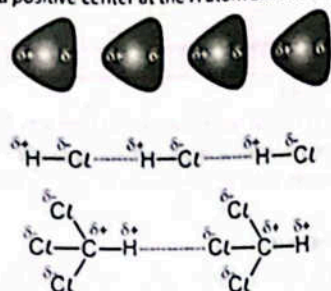
Figure: Permanent dipole-permanent dipole forces in HCl and chloroform
