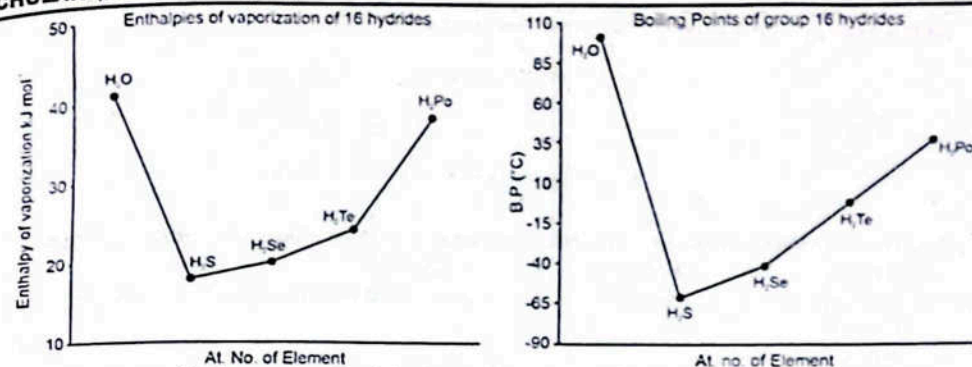
Figure: A graphical expression of variation in enthalpy of vaporization and B.P.s of group 16 hydrides. With the increasing atomic size down the group, from S to Po, the van der Waals forces also become stronger. If water had followed this trend, the heat of vaporization of water would be the lowest among the group members.
