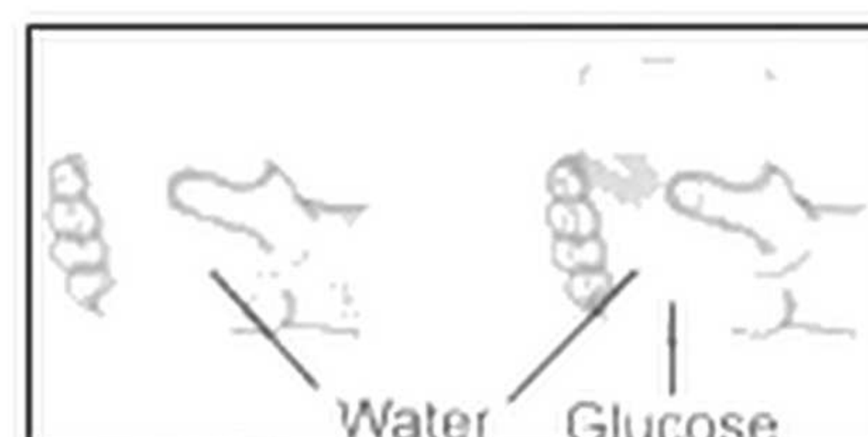
Figure 5.8: Heat is taken in when glucose dissolves in water.
