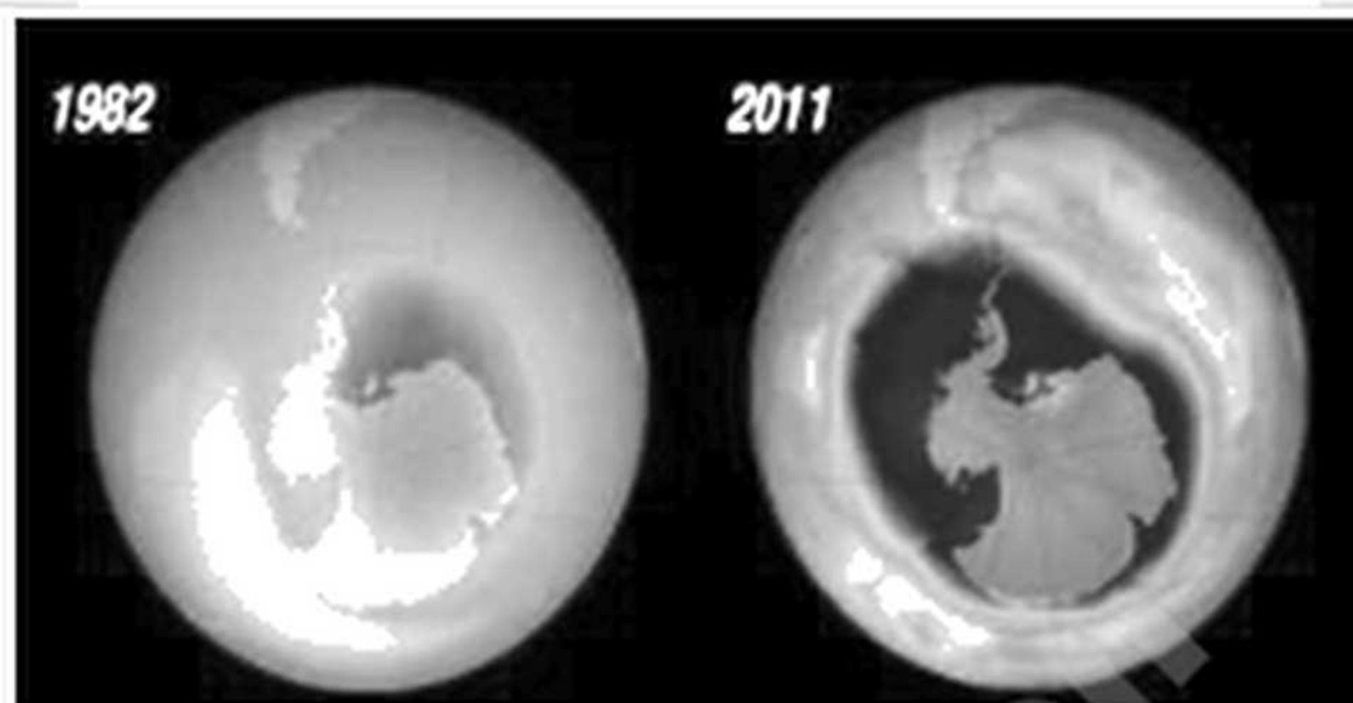
Figure 4.5: Ozone depletion
