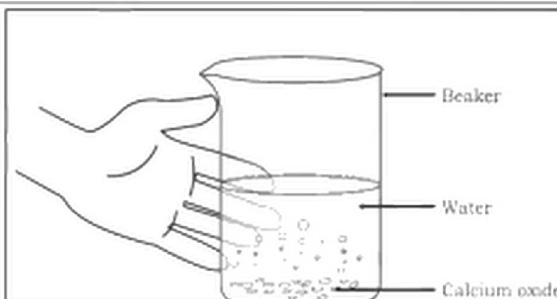
Figure 5.4: Combination reaction
