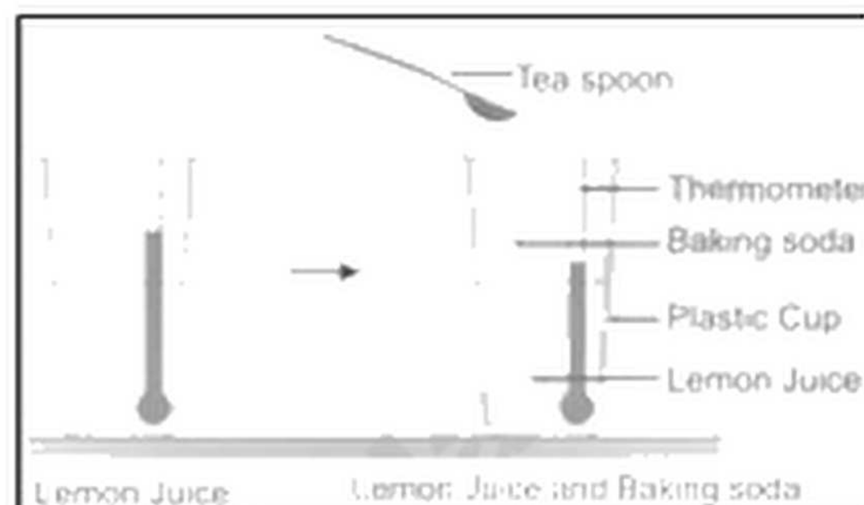
Figure 5.7: Endothermic reaction
