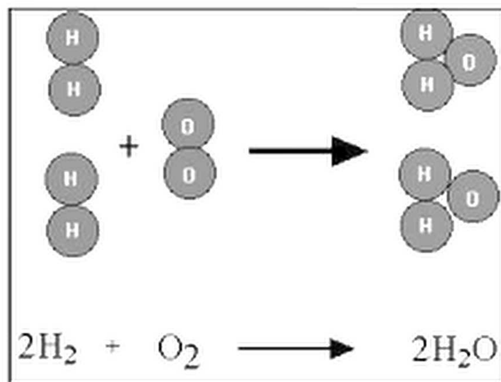
Figure 5.2: The bonds in the diatomic molecule of \text{H}_2 (hydrogen) and \text{O}_2 (oxygen) are broken, and new bonds are formed between hydrogen and oxygen atom
