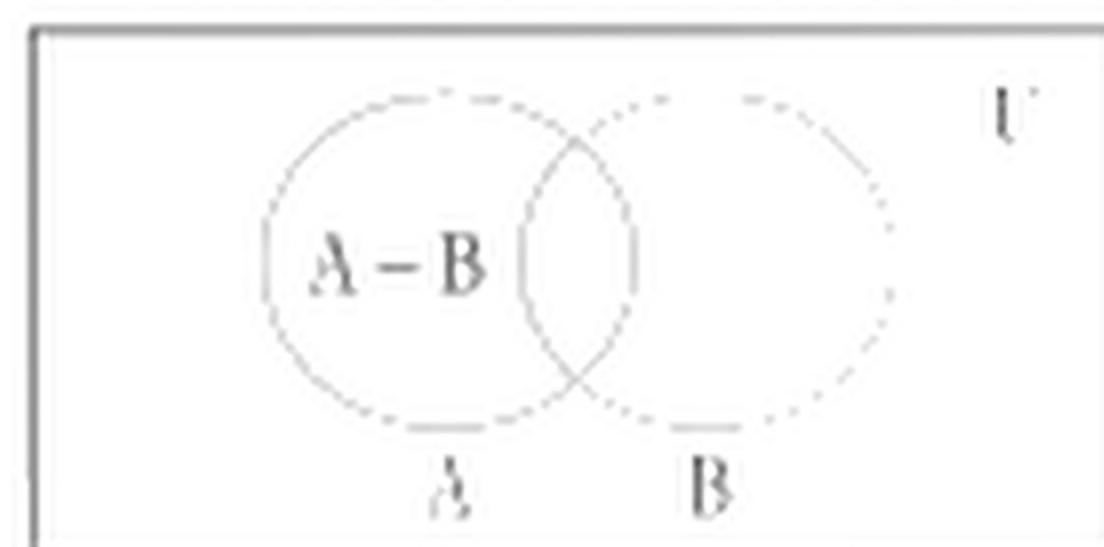
Different of two sets A - B
